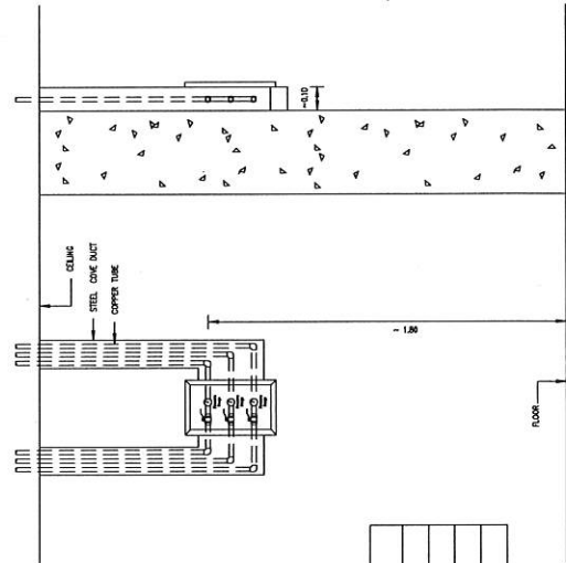
TYPICAL DETAIL FOR ZONE VALVE (THREE SYSTEM)
